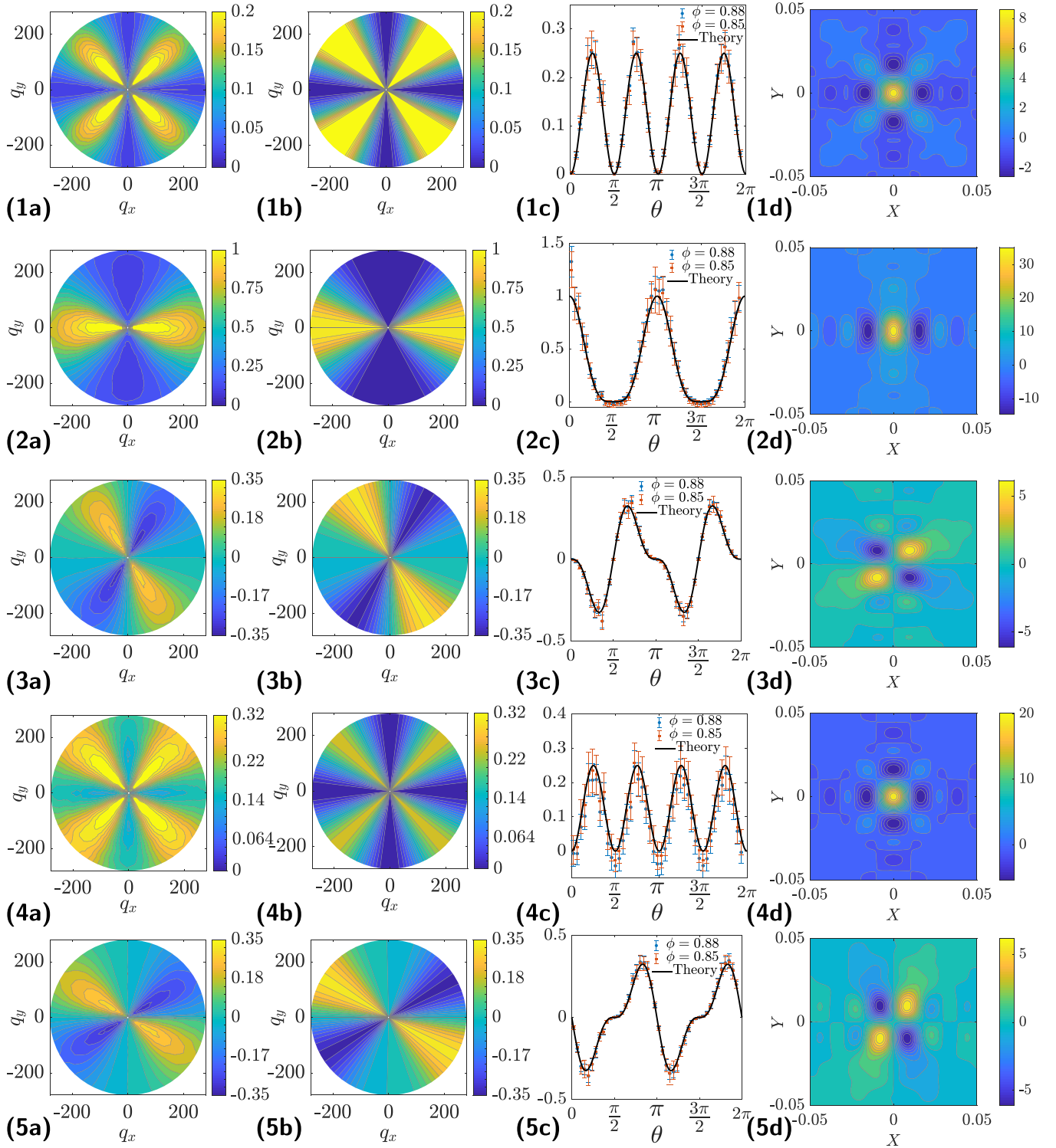
FIG. 5. Comparison of the correlation functions obtained from numerical simulations with the theoretical predictions, in 2D. The comparisons given, are for a system of 8 192 grains at two packing fractions \phi = 0.88 and \phi = 0.85 . The four columns show, respectively: (a) the numerical results in q space, (b) the theoretical predictions in q space, (c) quantitative comparison between the radially averaged (integrated over |q| ) correlations, plotted as a function of the angle \theta , and (d) the numerical results in real space obtained by an inverse Fourier transform of the correlations in Fourier space. The modulations seen in panel (d) are at the grain scale. The contour plots are for \phi = 0.88 and the quantitative comparison in the third column shows the results for both \phi = 0.85 and \phi = 0.88 . In the quantitative comparison plots, the data has been scaled by the maximum value of the angular C_{xxxx} correlation function. Each row presents the results for a specific correlation function. The five rows present, respectively: (1) C_{xyxy} , (2) C_{yyyy} , (3) C_{xxyx} , (4) C_{xxyy} , and (5) C_{xyyy} whose explicit forms are given in the Appendix [see Eq. (A27)].
