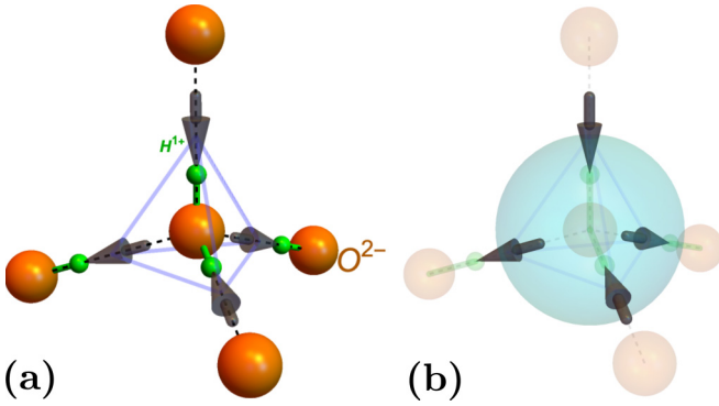
FIG. 2. Emergent electromagnetism in hexagonal phase of water-ice and spin ice: (a) In the hexagonal phase of ice-crystals each O^{2-} ion has four H^{1+} ion (proton) along the O-O bonds with two being near and two being far that gives rise to the six possible configuration one of which is shown, in accordance with Bernal-Fowler ice rules [39] or 2-in-2-out rules in terms of the displacement of the proton from the mid-point of the O-O bond shown in arrows. (b) The arrows are mapped to an emergent magnetic field \mathbf{b} , such that the ice rules implement its zero divergence, \nabla \cdot \mathbf{b} = 0 . The low-energy description is in terms of an emergent magnetostatics which does not depend on any specific configuration of the protons (see text for details).
