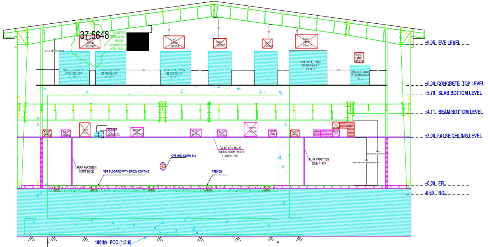
VIEW B-B
