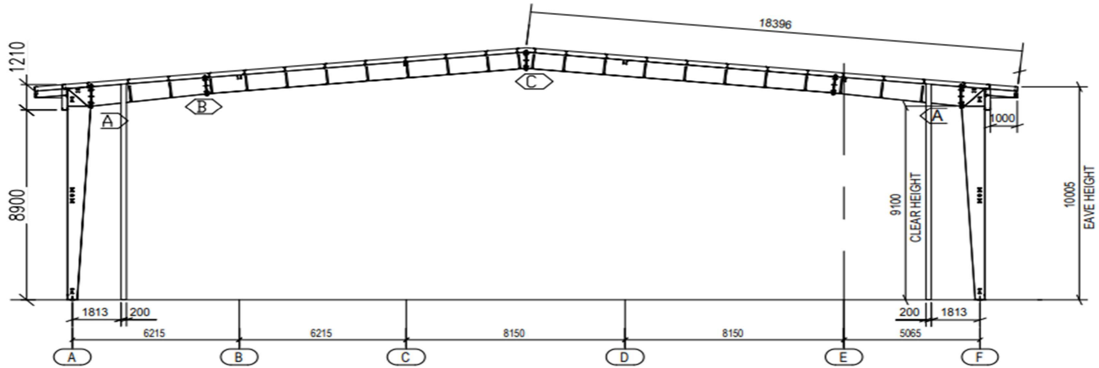
CROSS SECTION ALONG GRID-8 to 10
