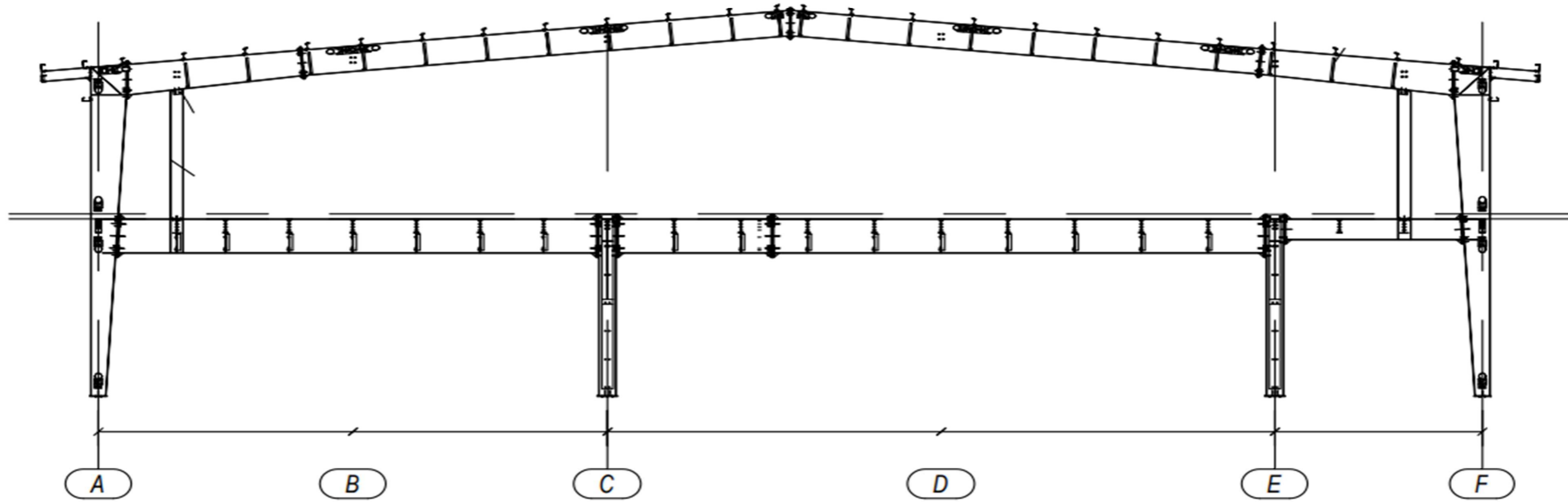
CROSS SECTION FORM GRID 6 TO 7
