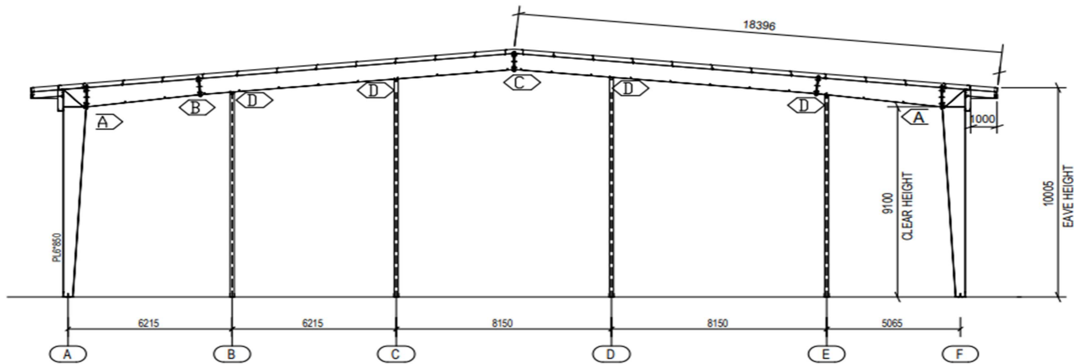
CROSS SECTION ALONG GRID - 11
