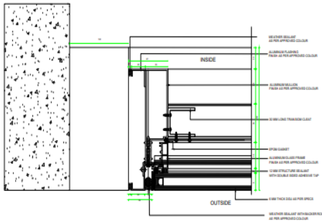
TYPICAL END DETAIL
