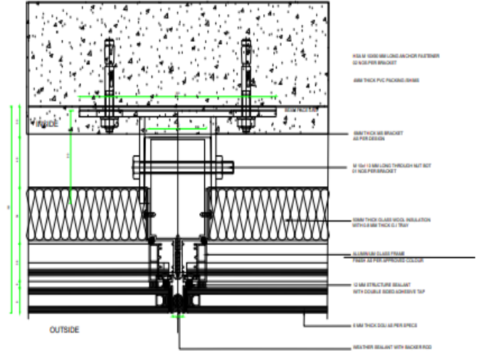
TYPICAL INTERMEDIATE DETAIL AT BEAM LVL
