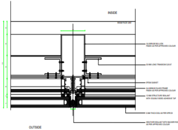
TYPICAL INTERMEDIATE DETAIL AT VISION LVL
